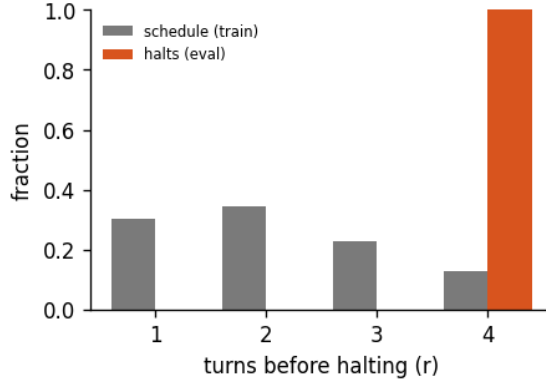
Figure 2: Halting distribution: the fraction of forward passes that stop after r turns, for the 4-turn recurrent loop of run calm-e, early-halt rate 0%, mean boundary KL 36.1. schedule is the random loop-count the model trains under; halts is where the KL gate actually stops at inference. A mass pinned at the maximum (KL never collapsing) is the honest signature of a model that has not yet learned to converge early - the decision is real, not yet decisive.
