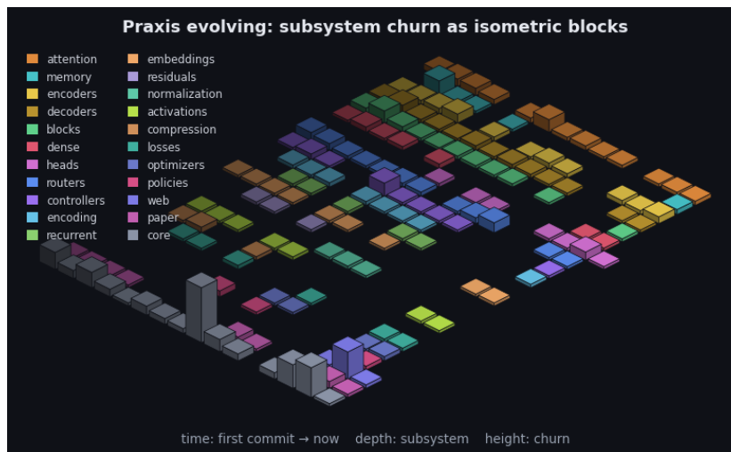
Figure 7: Praxis’s git history as an isometric block field over the last 2209 commits: each block is one subsystem’s line churn in one time window (time runs front-right toward HEAD, subsystem into depth, block height is churn). Blocks dim toward the past - the recency kernel the model applies to a sequence, turned on the repository. By recency-weighted churn the current center of gravity is core, web, encoders. The framework charts the hand that builds it.
