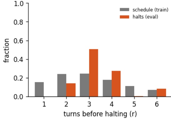
Figure 8: Halting distribution: the fraction of forward passes that stop after r turns, for the 6-turn recurrent loop of run abstractinator-h, early-halt rate 28%, mean boundary KL 0.241. schedule is the random loop-count the model trains under; halts is where the KL gate actually stops at inference. A mass pinned at the maximum (KL never collapsing) is the honest signature of a model that has not yet learned to converge early - the decision is real, not yet decisive.
