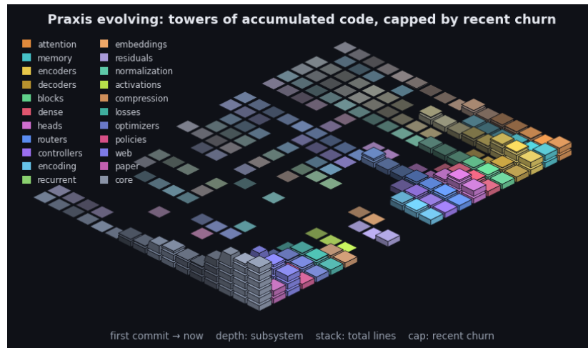
Figure 12: Praxis's git history as an isometric terrain over the last 2443 commits. Each cell is one subsystem in one time window: a stack of base blocks for its accumulated size (total lines, recency-weighted) topped by a vivid cap for that window's line churn - the standing codebase carrying the recent activity. Both are weighted by recency (the kernel the model applies to a sequence, turned on the repository): recent windows stack tall with bright caps while history thins toward the always-present prior - the low valley we roll into. Color fades from each subsystem's hue toward a neutral prior into the past, banded in phased strata over a non-linear timescale. It is the bias/variance geometry read along the frequency axis (see the project notes): loud recent corrections over the quiet, ever-present base. By recency-weighted churn the current center of gravity is core, web, paper. The framework charts the hand that builds it.
