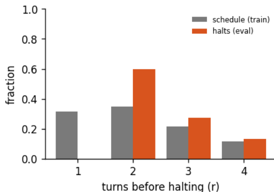
Figure 8: Halting distribution: the fraction of forward passes that stop after r turns, for the 4-turn recurrent loop of run abstractinator-f, early-halt rate 36%, mean boundary KL 0.368. schedule is the random loop-count the model trains under; halts is where the KL gate actually stops at inference. A mass pinned at the maximum (KL never collapsing) is the honest signature of a model that has not yet learned to converge early - the decision is real, not yet decisive.
