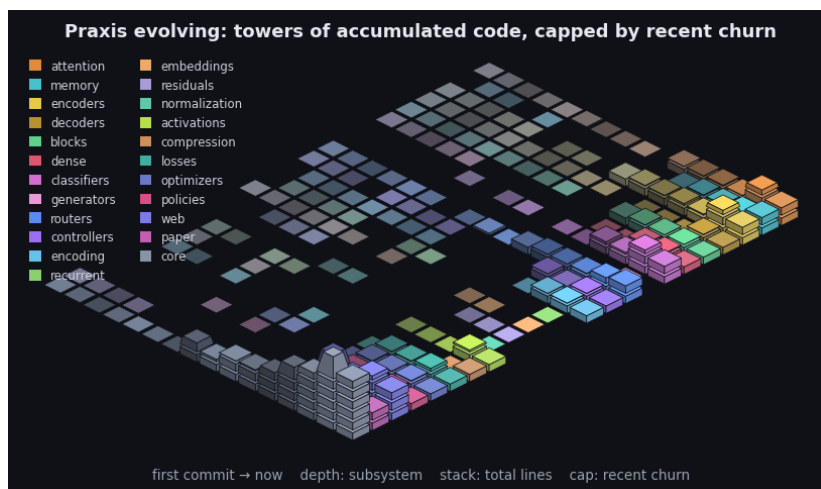
Figure 13: Praxis’s git history as an isometric terrain over the last 2650 commits. Each cell is one subsystem in one time window: a stack of base blocks for its accumulated size (total lines, recency-weighted) topped by a vivid cap for that window’s line churn - the standing codebase carrying the recent activity. Both are weighted by recency (the kernel the model applies to a sequence, turned on the repository): recent windows stack tall with bright caps while history thins toward the always-present prior - the low valley we roll into. Color fades from each subsystem’s hue toward a neutral prior into the past, banded in phased strata over a non-linear timescale. It is the bias/variance geometry read along the frequency axis (see the project notes): loud recent corrections over the quiet, ever-present base. By recency-weighted churn the current center of gravity is core, web, encoders. The framework charts the hand that builds it.
