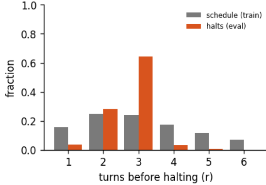
Figure 9: Halting distribution: the fraction of forward passes that stop after r turns, for the 6-turn recurrent loop of run byte-latent-a, early-halt rate 37%, mean boundary KL 0.0161. schedule is the random loop-count the model trains under; halts is where the KL gate actually stops at inference. A mass pinned at the maximum (KL never collapsing) is the honest signature of a model that has not yet learned to converge early - the decision is real, not yet decisive.
