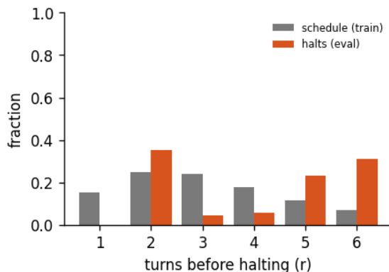
Figure 8: Halting distribution: the fraction of forward passes that stop after r turns, for the 6-turn recurrent loop of run abstractinator-r, early-halt rate 18%, mean boundary KL 0.509. schedule is the random loop-count the model trains under; halts is where the KL gate actually stops at inference. A mass pinned at the maximum (KL never collapsing) is the honest signature of a model that has not yet learned to converge early - the decision is real, not yet decisive.
