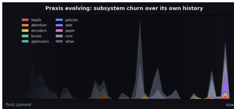
Figure 6: Per-subsystem line churn across the last 2207 commits of Praxis’s git history, binned over time (left = first commit, right = now). The distant past fades: strength is decayed by distance from HEAD - the same recency kernel the model applies to a sequence, turned on the repository. By recency-weighted churn the current center of gravity is other, core, web. The framework charts the hand that builds it.
