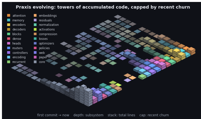
Figure 4: Praxis’s git history as an isometric terrain over the last 2274 commits. Each cell is one subsystem in one time window: a stack of base blocks for its accumulated size (total lines, recency-weighted) topped by a vivid cap for that window’s line churn - the standing codebase carrying the recent activity. Both are weighted by recency (the kernel the model applies to a sequence, turned on the repository): recent windows stack tall with bright caps while history thins toward the always-present prior - the low valley we roll into. Color fades from each subsystem’s hue toward a neutral prior into the past, banded in phased strata over a non-linear timescale. It is the bias/variance geometry read along the frequency axis (see the project notes): loud recent corrections over the quiet, ever-present base. By recency-weighted churn the current center of gravity is core, web, encoders. The framework charts the hand that builds it.
