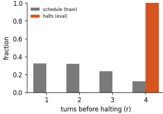
Figure 2: Halting distribution: the fraction of forward passes that stop after r turns, for the 4-turn recurrent loop of run calm-d, early-halt rate 0%, mean boundary KL 66.7. schedule is the random loop-count the model trains under; halts is where the KL gate actually stops at inference. A mass pinned at the maximum (KL never collapsing) is the honest signature of a model that has not yet learned to converge early - the decision is real, not yet decisive.
