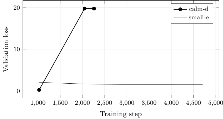
Figure 5: Validation Loss across the 2 most recent experiments with comparable validation curves; the leading run (calm-d) is drawn in bold. Generated from run logs - metrics that are not comparable across families (token loss vs. byte bits-per-byte vs. codec/CALM BrierLM) are excluded by construction, so the curves on this axis mean the same thing.
