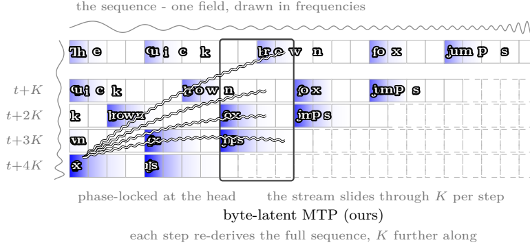
Figure 4: The fox at every step: the strip of Figure 6, reorganized as this head reads it. Top: the sequence, its field drawn in frequencies. The spaces stay in the lattice as teeth - byte-wide white cells holding no content, pure entropy: the boundaries byte-latent patching cuts on. Below: successive MTP steps. A step advances the stream K bytes and re-derives the full sequence from its new head, so each row is the whole sequence again, slid K left - never a K -byte fragment (dashed cells: not yet written). Density is per patch, heaviest at a patch’s first byte and decaying through its predictable tail all the way to white - every patch keeps a white stretch where genuinely little information lives - and the characters melt out of their boxes the same way, pooling toward each patch’s head, spilling over the cell walls, leaving the right of every window sparse - and they crowd further left with every step, each patch compressing toward its own head until the last row holds each patch’s bytes stacked on a single position. Each step runs denser than the last as context accumulates, and every row darkens along T , because later positions compress the full sequence so far, however many tokens remain to attend to; the final row runs densest of all, its white regions narrowest - information densifying as it twists toward the final representation, t+4K . The outlined band is a fixed K -wide window: the stream slides through it, one column of K per step - in standard byte-latent decoding it would advance one cell at a time. The wiggly strands run from the window’s last content byte, at every earlier step, to the first token of the final sequence - the one they all resolve into, so it draws no strand of its own: every window is connected to both the future and the past of every sequence - phase-locking, every feature contributing to every representation. The locking runs down the depth axis too - the vertical wave at the left is the same field read across the steps, humming at the trunk, chirping into t+4K . One byte still traces a diagonal through the succession of views, K cells left per step, re-predicted and bolstered or refuted at every pass. Schematic (drawn at K=4 ; the mechanism is K -generic), not measured; the measured object is the per-depth acceptance profile.
