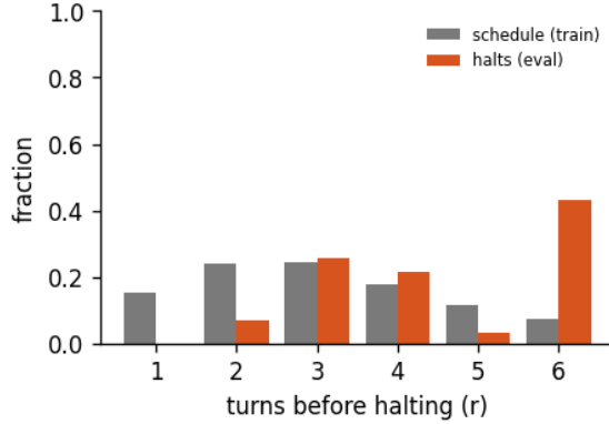
Figure 8: Halting distribution: the fraction of forward passes that stop after r turns, for the 6-turn recurrent loop of run abstractinator-h, early-halt rate 14%, mean boundary KL 0.29. schedule is the random loop-count the model trains under; halts is where the KL gate actually stops at inference. A mass pinned at the maximum (KL never collapsing) is the honest signature of a model that has not yet learned to converge early - the decision is real, not yet decisive.
