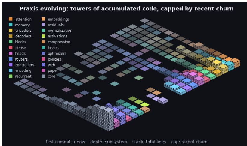
Figure 12: Praxis’s git history as an isometric terrain over the last 2466 commits. Each cell is one subsystem in one time window: a stack of base blocks for its accumulated size (total lines, recency-weighted) topped by a vivid cap for that window’s line churn - the standing codebase carrying the recent activity. Both are weighted by recency (the kernel the model applies to a sequence, turned on the repository): recent windows stack tall with bright caps while history thins toward the always-present prior - the low valley we roll into. Color fades from each subsystem’s hue toward a neutral prior into the past, banded in phased strata over a non-linear timescale. It is the bias/variance geometry read along the frequency axis (see the project notes): loud recent corrections over the quiet, ever-present base. By recency-weighted churn the current center of gravity is core, web, paper. The framework charts the hand that builds it.
