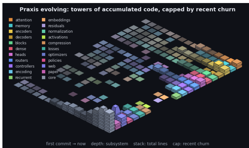
Figure 4: Praxis’s git history as an isometric terrain over the last 2338 commits. Each cell is one subsystem in one time window: a stack of base blocks for its accumulated size (total lines, recency-weighted) topped by a vivid cap for that window’s line churn - the standing codebase carrying the recent activity. Both are weighted by recency (the kernel the model applies to a sequence, turned on the repository): recent windows stack tall with bright caps while history thins toward the always-present prior - the low valley we roll into. Color fades from each subsystem’s hue toward a neutral prior into the past, banded in phased strata over a non-linear timescale. It is the bias/variance geometry read along the frequency axis (see the project notes): loud recent corrections over the quiet, ever-present base. By recency-weighted churn the current center of gravity is core, web, paper. The framework charts the hand that builds it.
