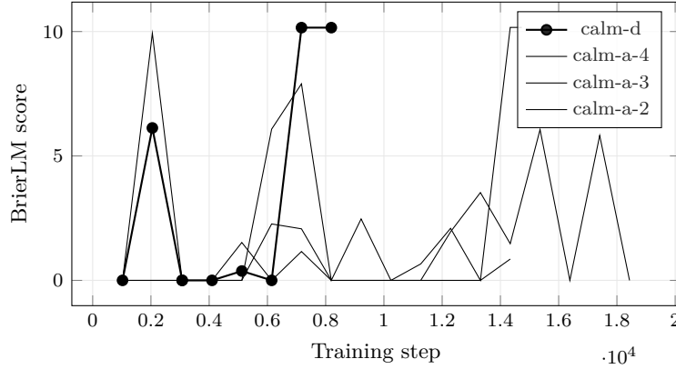
Figure 5: BrierLM across the 4 most recent experiments with comparable validation curves; the leading run (calm-d) is drawn in bold. Generated from run logs - metrics that are not comparable across families (token loss vs. byte bits-per-byte vs. codec/CALM BrierLM) are excluded by construction, so the curves on this axis mean the same thing.
