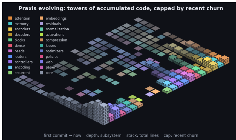
Figure 4: Praxis’s git history as an isometric terrain over the last 2278 commits. Each cell is one subsystem in one time window: a stack of base blocks for its accumulated size (total lines, recency-weighted) topped by a vivid cap for that window’s line churn - the standing codebase carrying the recent activity. Both are weighted by recency (the kernel the model applies to a sequence, turned on the repository): recent windows stack tall with bright caps while history thins toward the always-present prior - the low valley we roll into. Color fades from each subsystem’s hue toward a neutral prior into the past, banded in phased strata over a non-linear timescale. It is the bias/variance geometry read along the frequency axis (see the project notes): loud recent corrections over the quiet, ever-present base. By recency-weighted churn the current center of gravity is core, web, encoders. The framework charts the hand that builds it.
