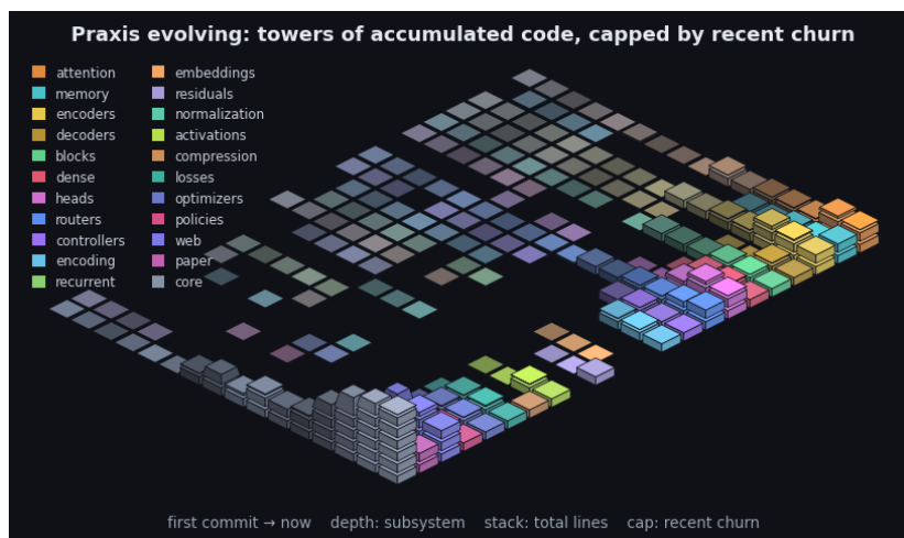
Figure 12: Praxis’s git history as an isometric terrain over the last 2544 commits. Each cell is one subsystem in one time window: a stack of base blocks for its accumulated size (total lines, recency-weighted) topped by a vivid cap for that window’s line churn - the standing codebase carrying the recent activity. Both are weighted by recency (the kernel the model applies to a sequence, turned on the repository): recent windows stack tall with bright caps while history thins toward the always-present prior - the low valley we roll into. Color fades from each subsystem’s hue toward a neutral prior into the past, banded in phased strata over a non-linear timescale. It is the bias/variance geometry read along the frequency axis (see the project notes): loud recent corrections over the quiet, ever-present base. By recency-weighted churn the current center of gravity is core, web, paper. The framework charts the hand that builds it.
