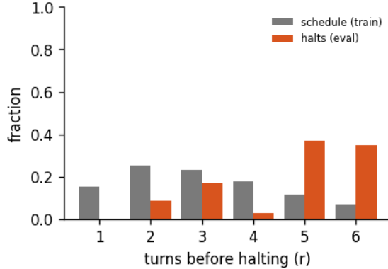
Figure 8: Halting distribution: the fraction of forward passes that stop after r turns, for the 6-turn recurrent loop of run abstractinator-v, early-halt rate 15%, mean boundary KL 0.309. schedule is the random loop-count the model trains under; halts is where the KL gate actually stops at inference. A mass pinned at the maximum (KL never collapsing) is the honest signature of a model that has not yet learned to converge early - the decision is real, not yet decisive.
