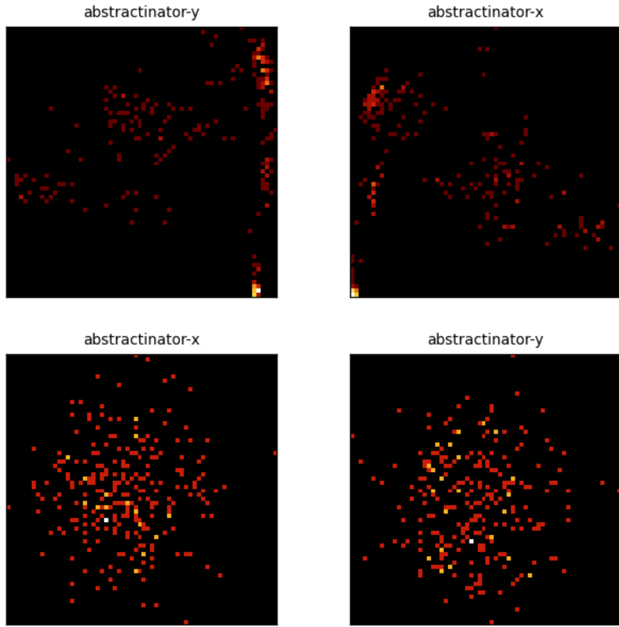
Figure 11: Center PCA density for the 4 most recent crystal-head runs (abstractinator-y, abstractinator-x, abstractinator-x, abstractinator-y). Each panel is the top-2 PCA projection of a head’s vocabulary centers, binned to a 64 \times 64 density grid (log color) - the same snapshot the dashboard renders live. Different runs settle into structurally different geometries, not noise.
