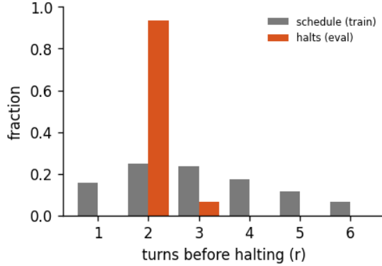
Figure 8: Halting distribution: the fraction of forward passes that stop after r turns, for the 6-turn recurrent loop of run abstractinator-y, early-halt rate 48%, mean boundary KL 0.517. schedule is the random loop-count the model trains under; halts is where the KL gate actually stops at inference. A mass pinned at the maximum (KL never collapsing) is the honest signature of a model that has not yet learned to converge early - the decision is real, not yet decisive.
