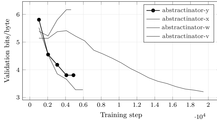
Figure 13: Bits per Byte across the 4 most recent experiments with comparable validation curves; the current experiment (abstractinator-y) is drawn in bold. Bold marks which run this build is reporting on , not which run scores best. The curves end wherever each run stopped, so they are at different points along their own training, and their endpoints are not a ranking. Generated from run logs - metrics that are not comparable across families (token loss vs. byte bits-per-byte vs. codec/CALM BrierLM) are excluded by construction, so the curves on this axis mean the same thing.
