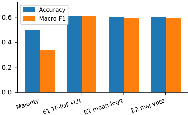
Outcome baselines, ILDC test (n=1,503)
