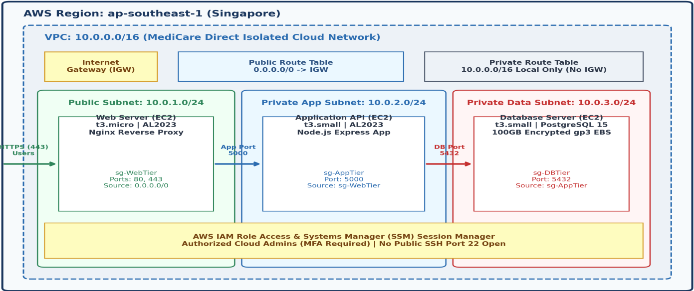
Figure 1: Complete AWS Architecture Diagram for MediCare Direct featuring VPC Subnet Segmentation, Routing, Security Groups, and IAM Governance.
