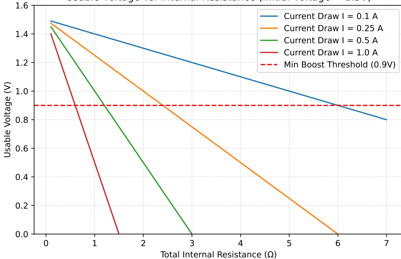
Usable Voltage vs. Internal Resistance (Initial Voltage = 1.5V)
