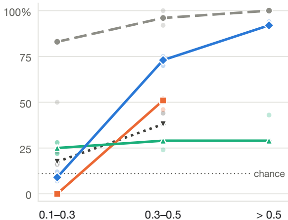
Forced choice, same-chapter (hit@1)
