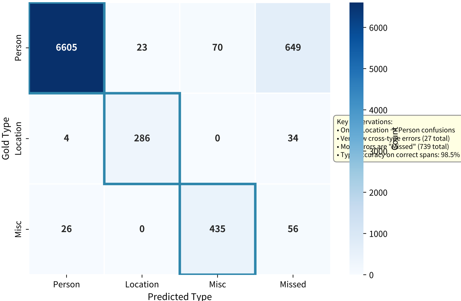
Type Confusion Matrix — Final NER (Low Cross-Type Confusion = Strong Semantic Understanding)
