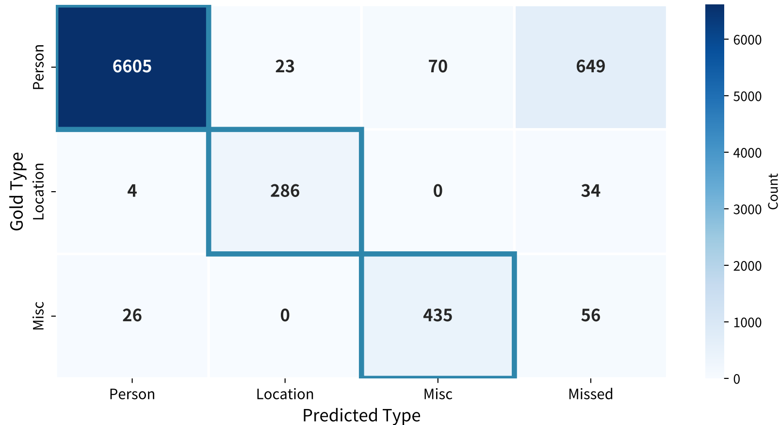
Type Confusion Matrix — Final NER (Low Cross-Type Confusion = Strong Semantic Understanding)
