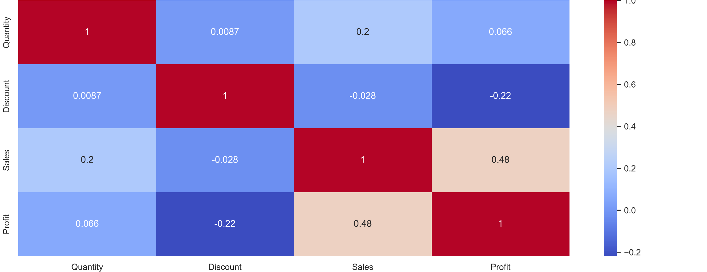
Correlation Matrix
