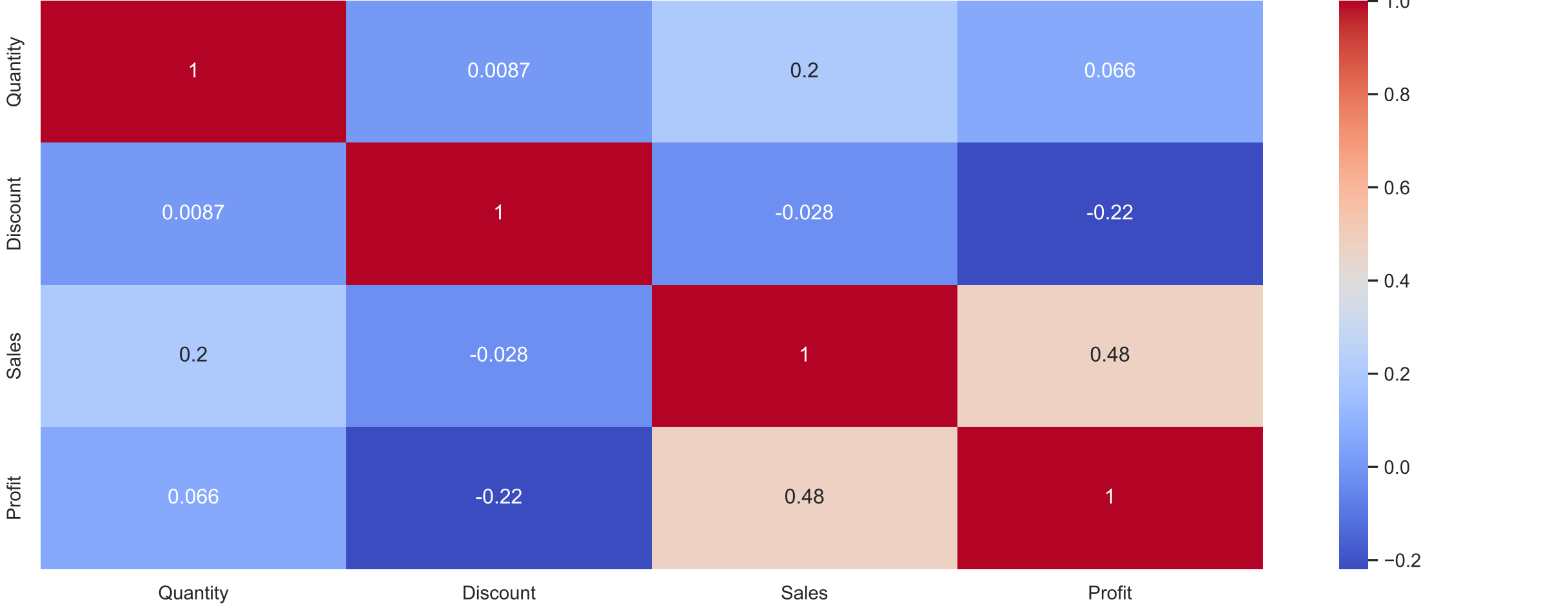
Correlation Matrix
