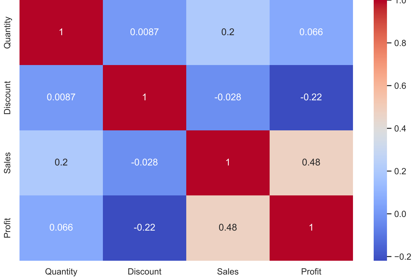
Correlation Matrix
