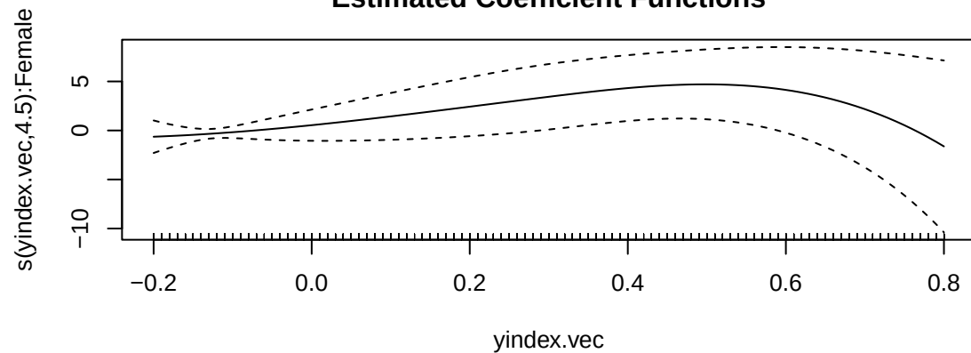
Estimated Coefficient Functions
