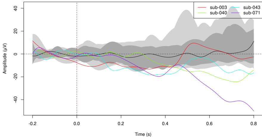
HDR Functional Boxplot, \alpha = (0.05, 0.50)
