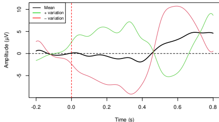
PC3 Perturbation (Expl. variance: 10.4%)
