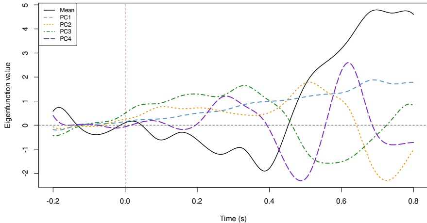
PCA Harmonics and Mean Function
