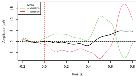
PC4 Perturbation (Expl. variance: 4.4%)
