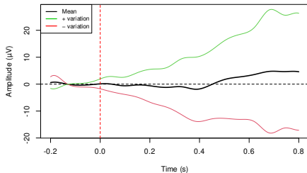
PC3 Perturbation (Expl. variance: 10.4%)
