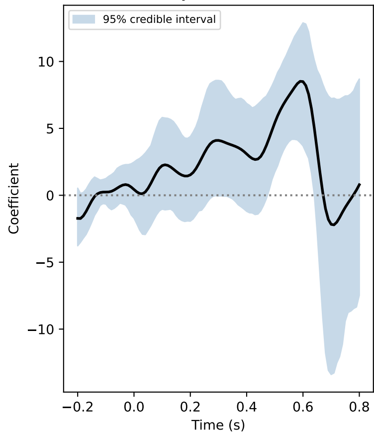
Bayes: Female
