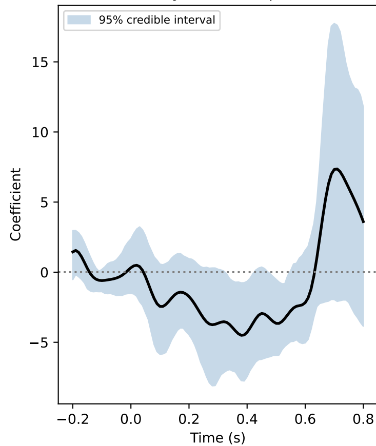
Bayes: Intercept
