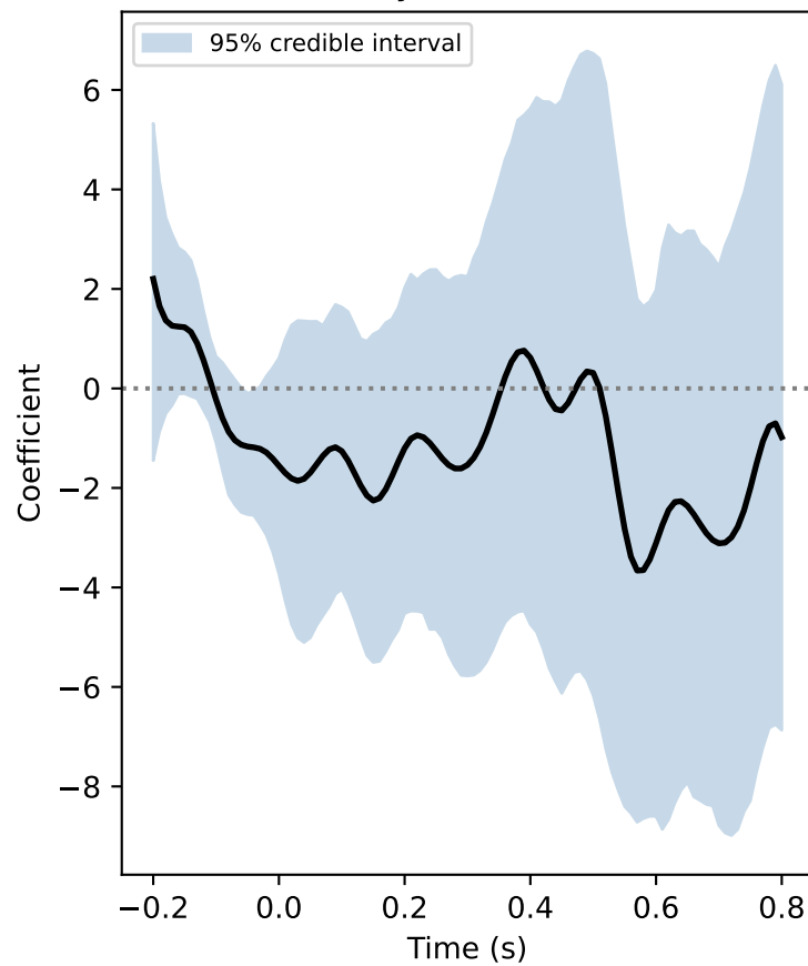
Bayes: ADHD
