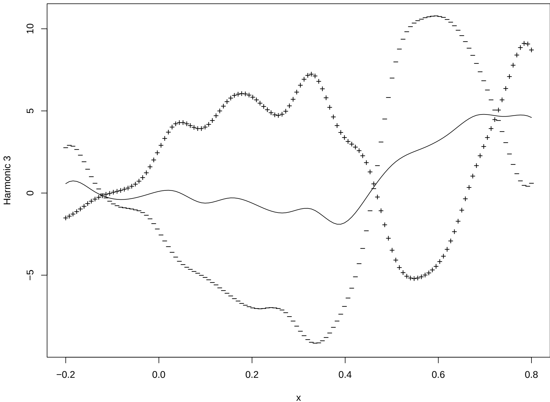
PCA function 3 (Percentage of variability 10.4 )
