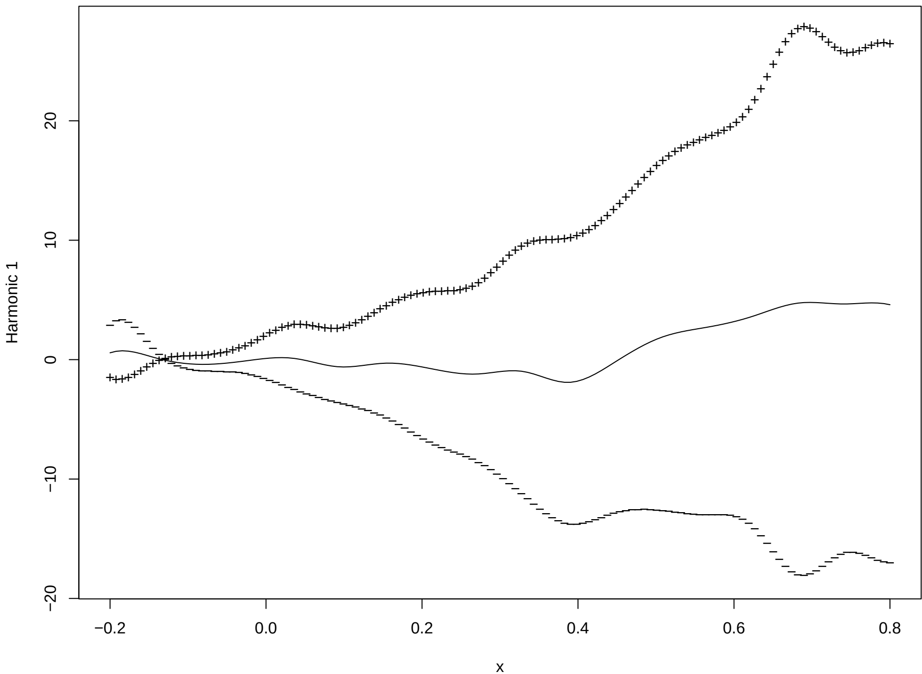
PCA function 1 (Percentage of variability 62.6 )
