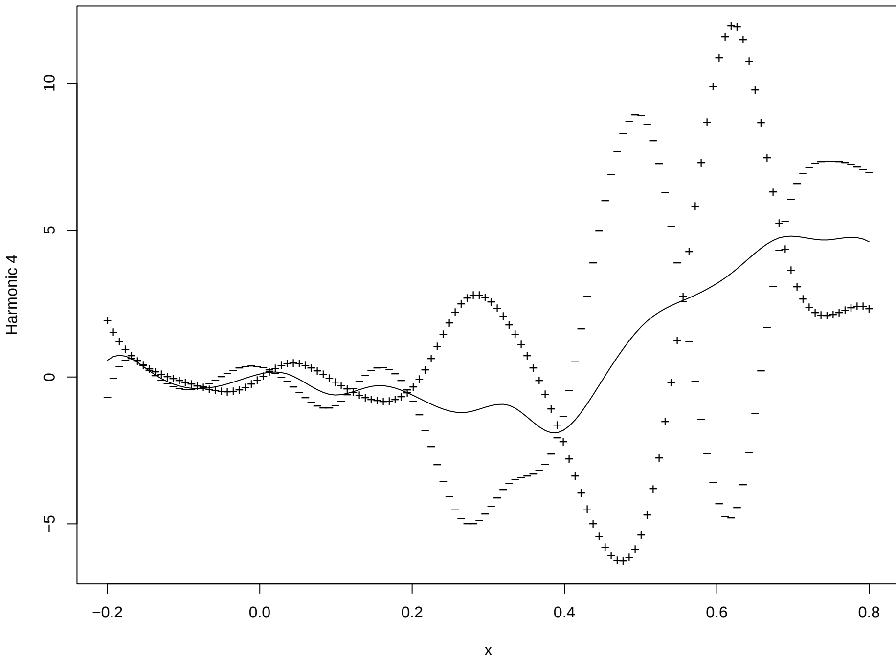
PCA function 4 (Percentage of variability 4.4 )
