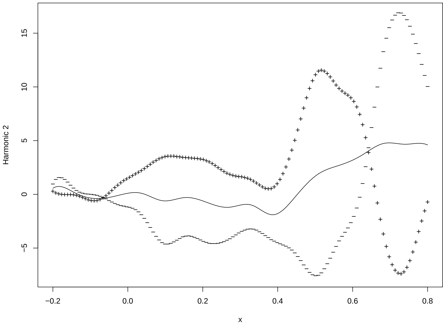
PCA function 2 (Percentage of variability 11.8 )
