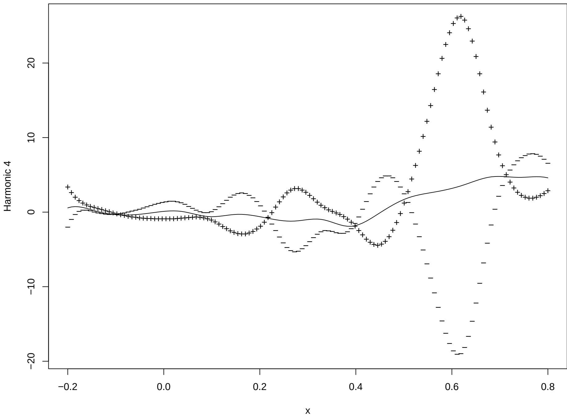
PCA function 4 (Percentage of variability 19.3 )
