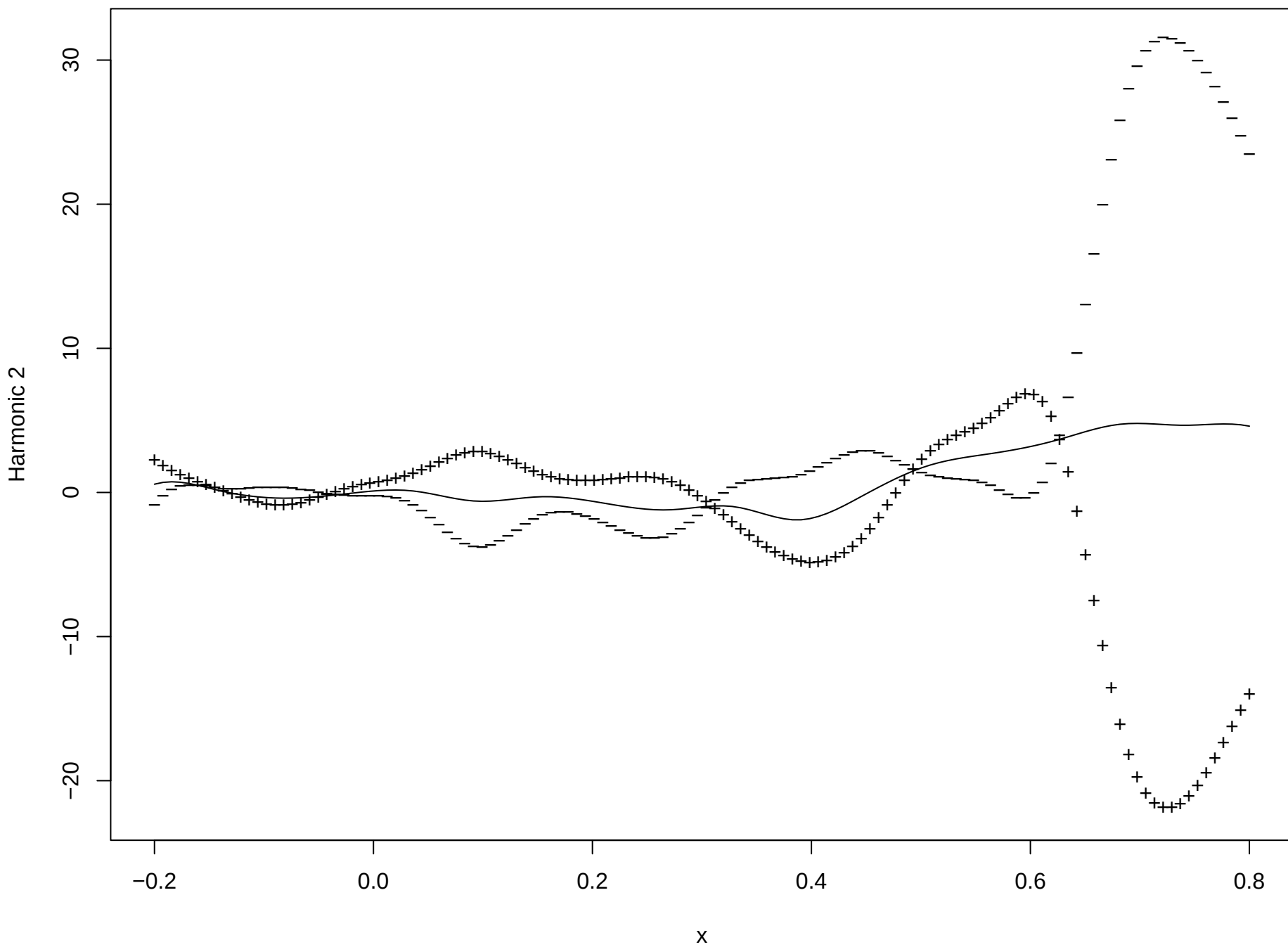
PCA function 2 (Percentage of variability 33.8 )
