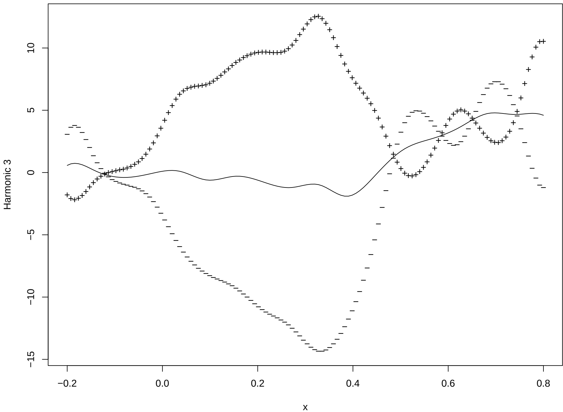
PCA function 3 (Percentage of variability 18.7 )
