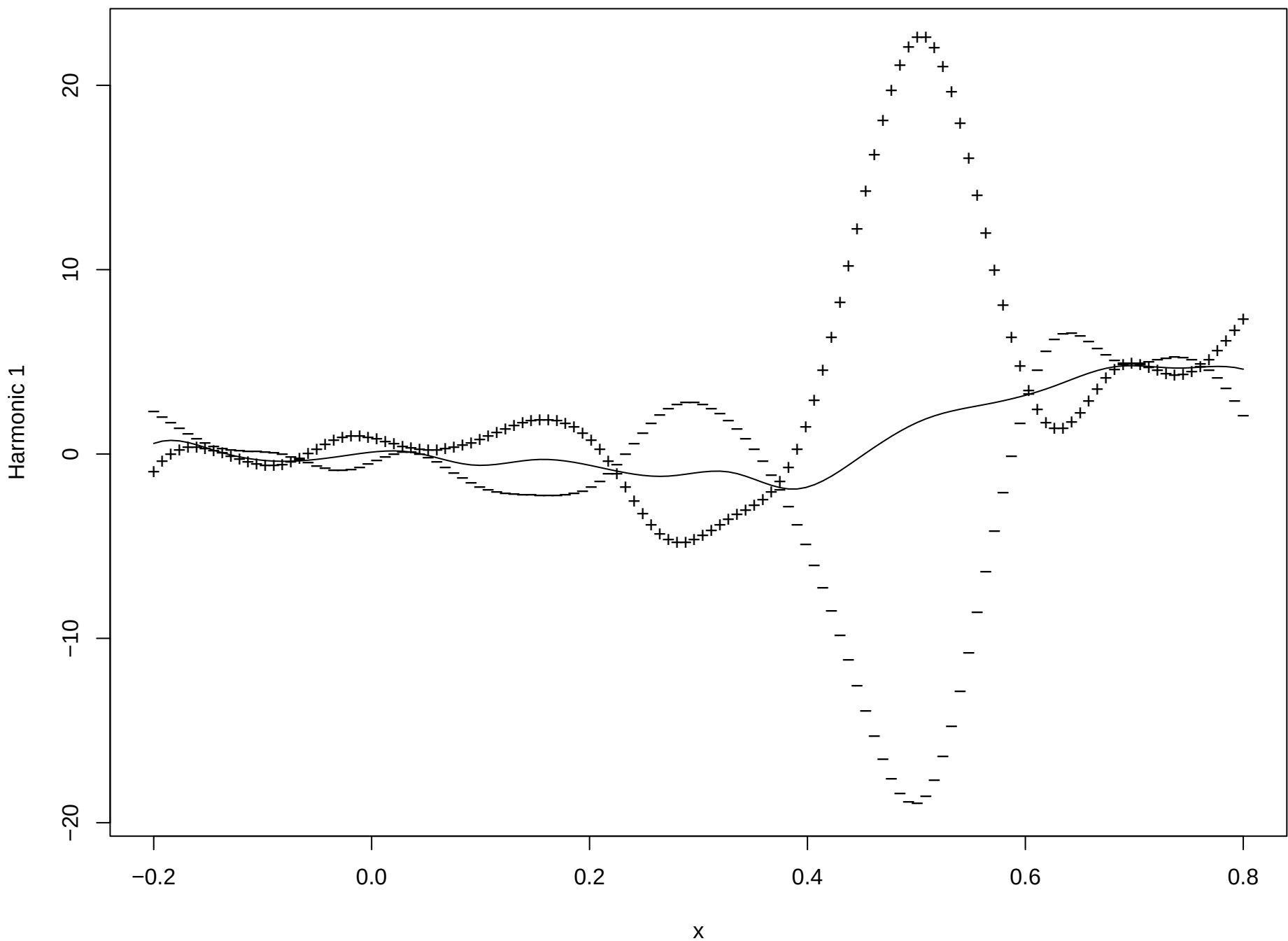
PCA function 1 (Percentage of variability 17.3 )
