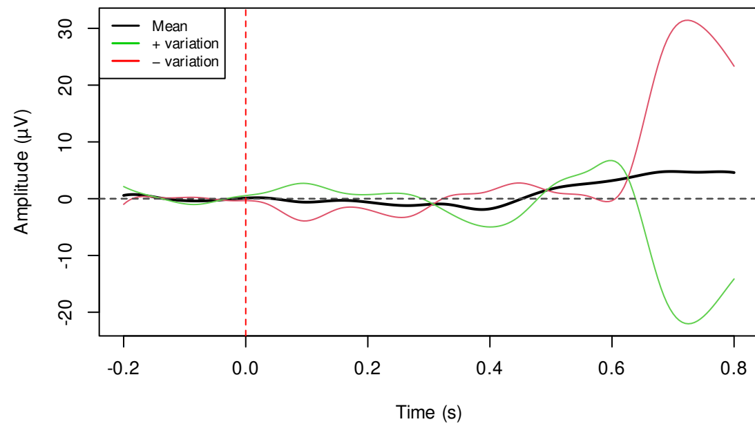
Rotated PC2 (Expl. variance: 33.8%)
