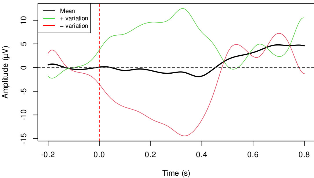
Rotated PC3 (Expl. variance: 18.7%)
