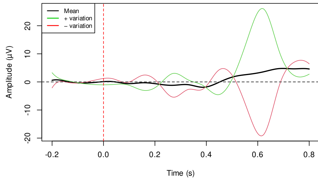
Rotated PC4 (Expl. variance: 19.3%)
