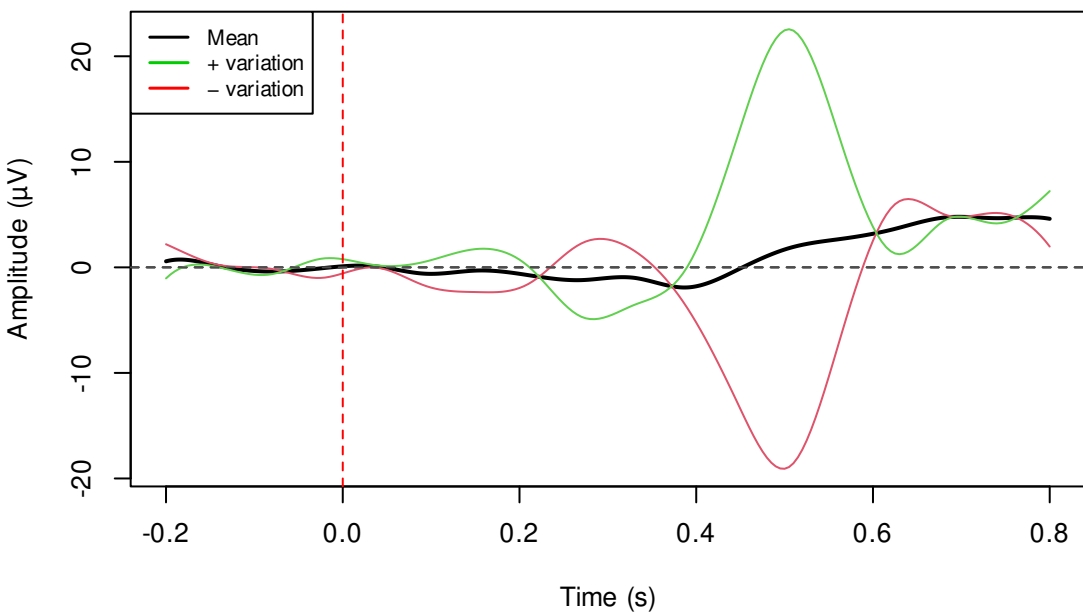
Rotated PC1 (Expl. variance: 17.3%)
