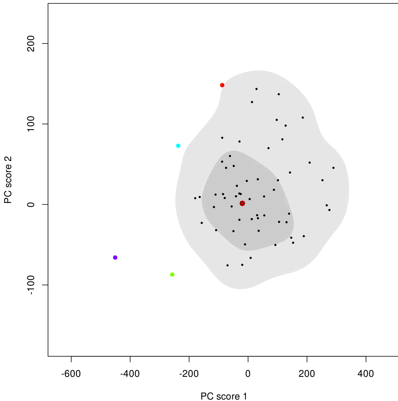
HDR Boxplot — Bivariate PCA Scores, \alpha = (0.05, 0.50)
