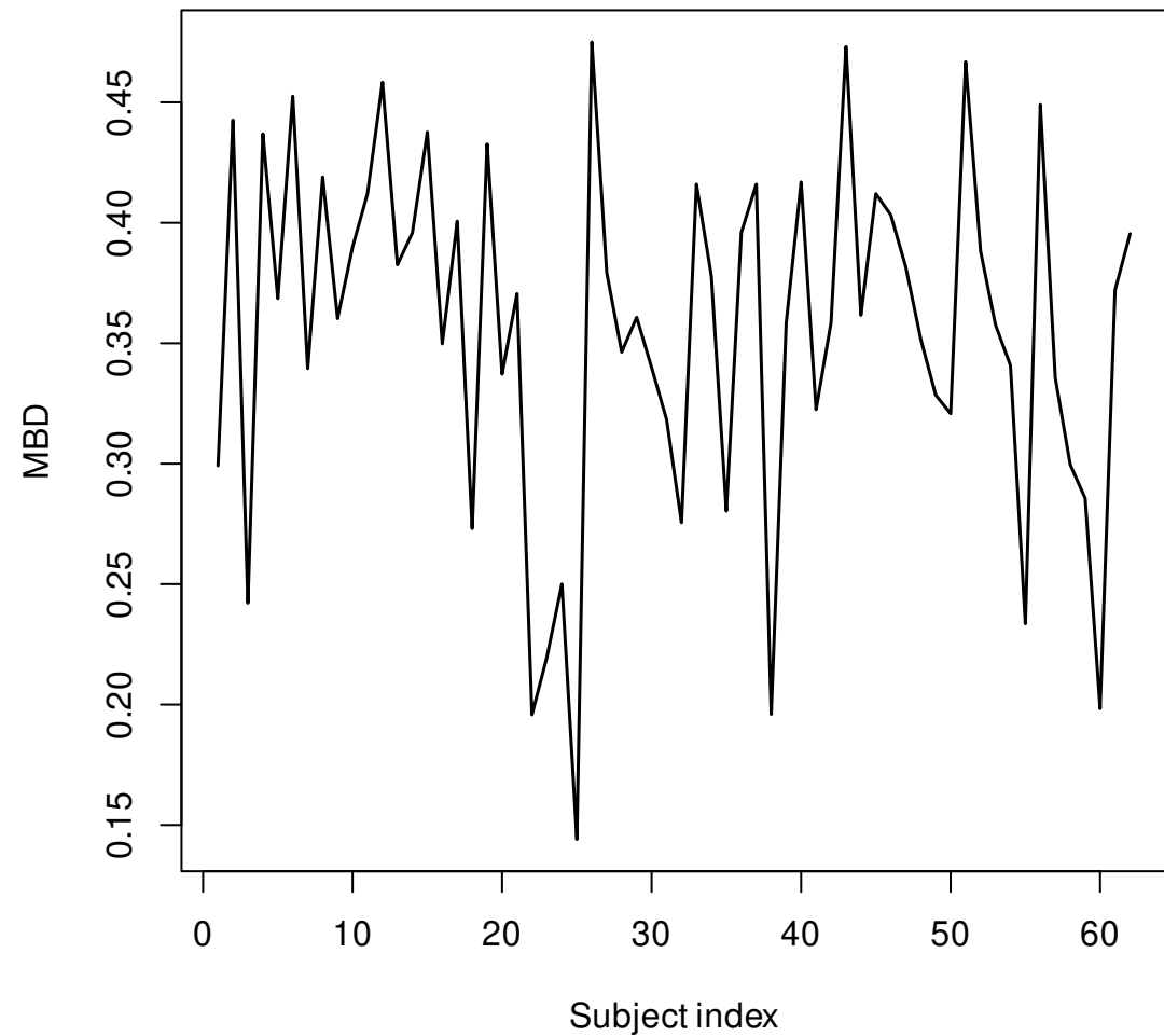
Modified Band Depth (MBD)
