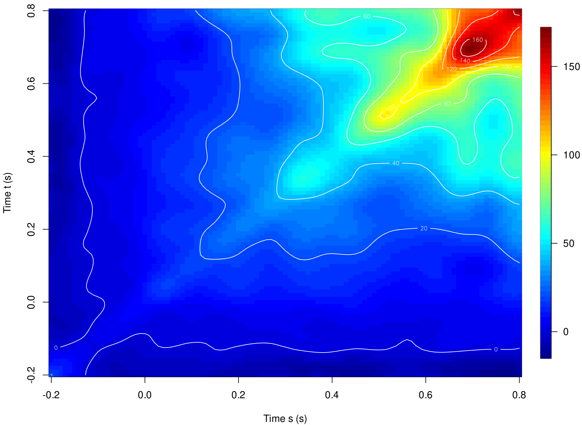
Covariance Surface
