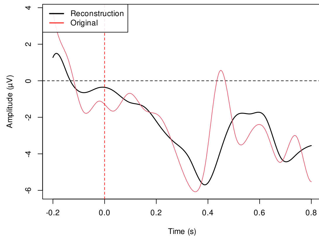
Subject sub-002 — 2 PCs
