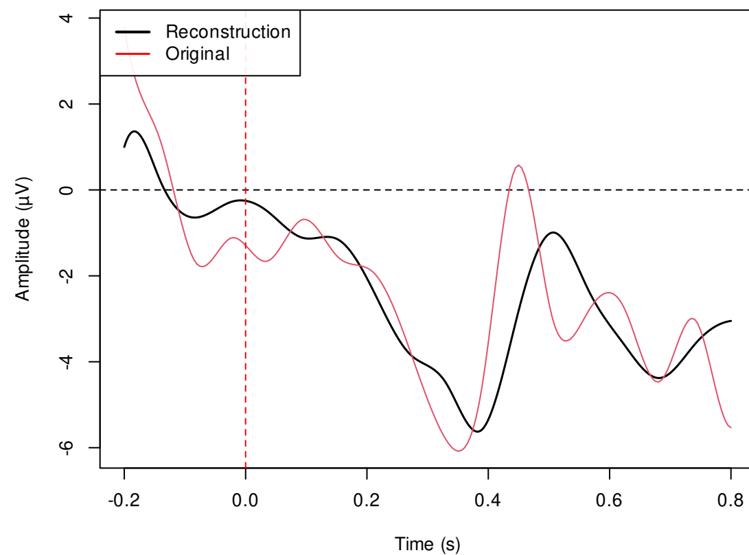
Subject sub-002 — 4 PCs
