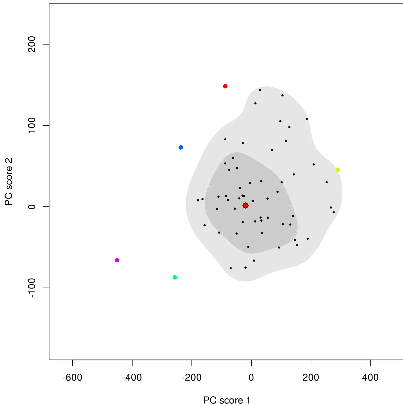
HDR Boxplot — Bivariate PCA Scores, \alpha = (0.07, 0.50)
