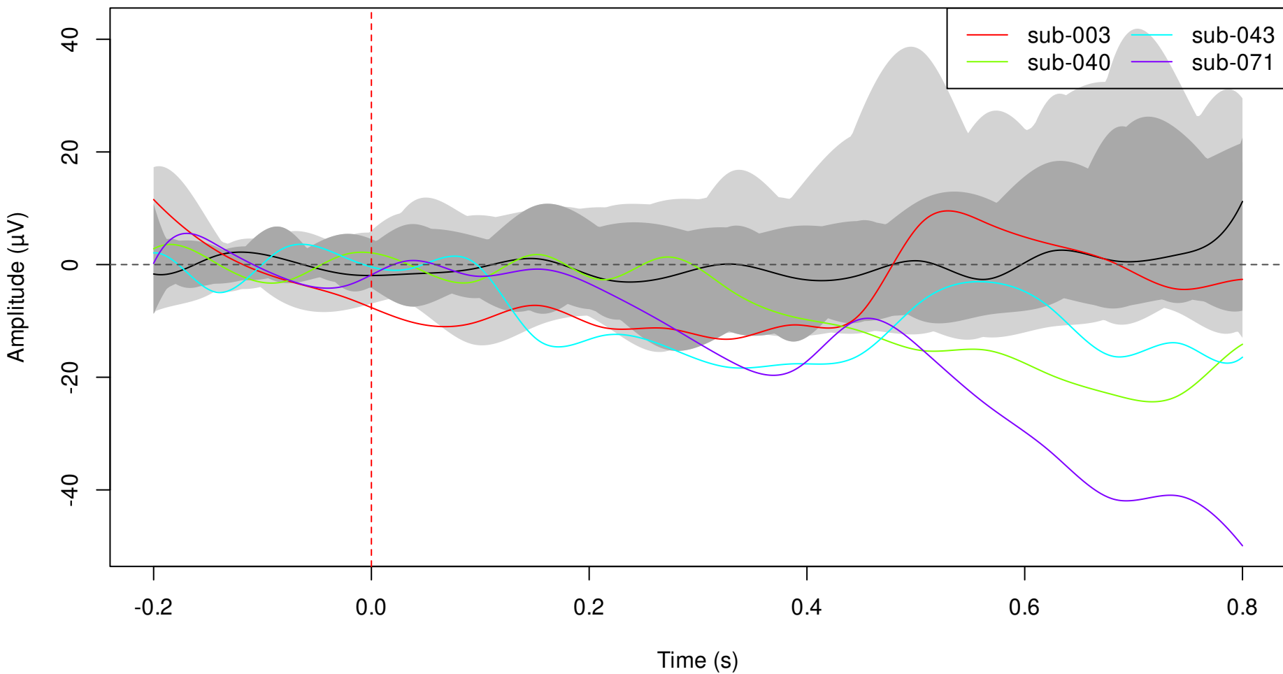
HDR Functional Boxplot, \alpha = (0.05, 0.50)
