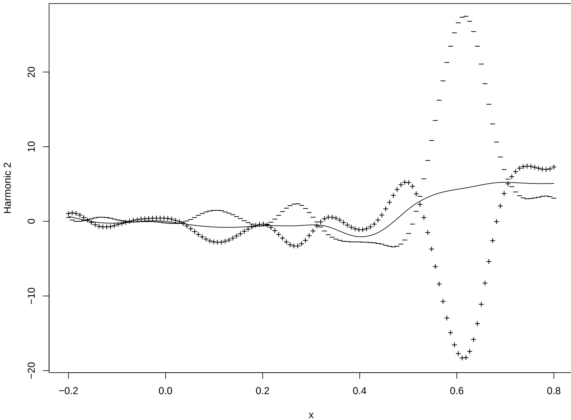
PCA function 2 (Percentage of variability 19 )
