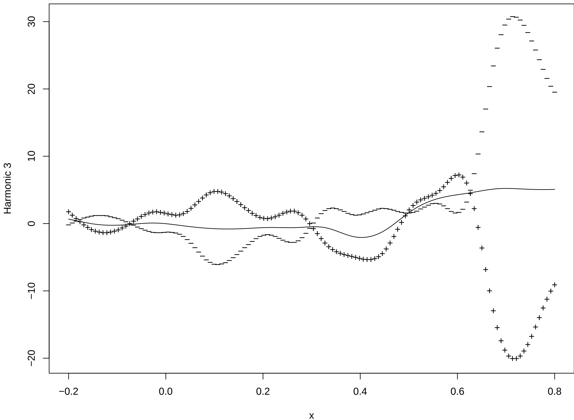
PCA function 3 (Percentage of variability 31.3 )
