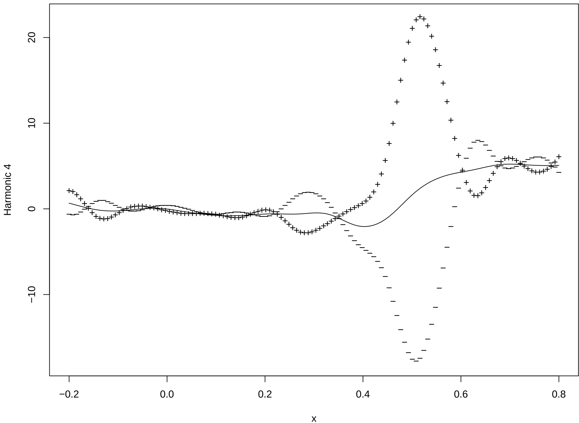
PCA function 4 (Percentage of variability 14.9 )
