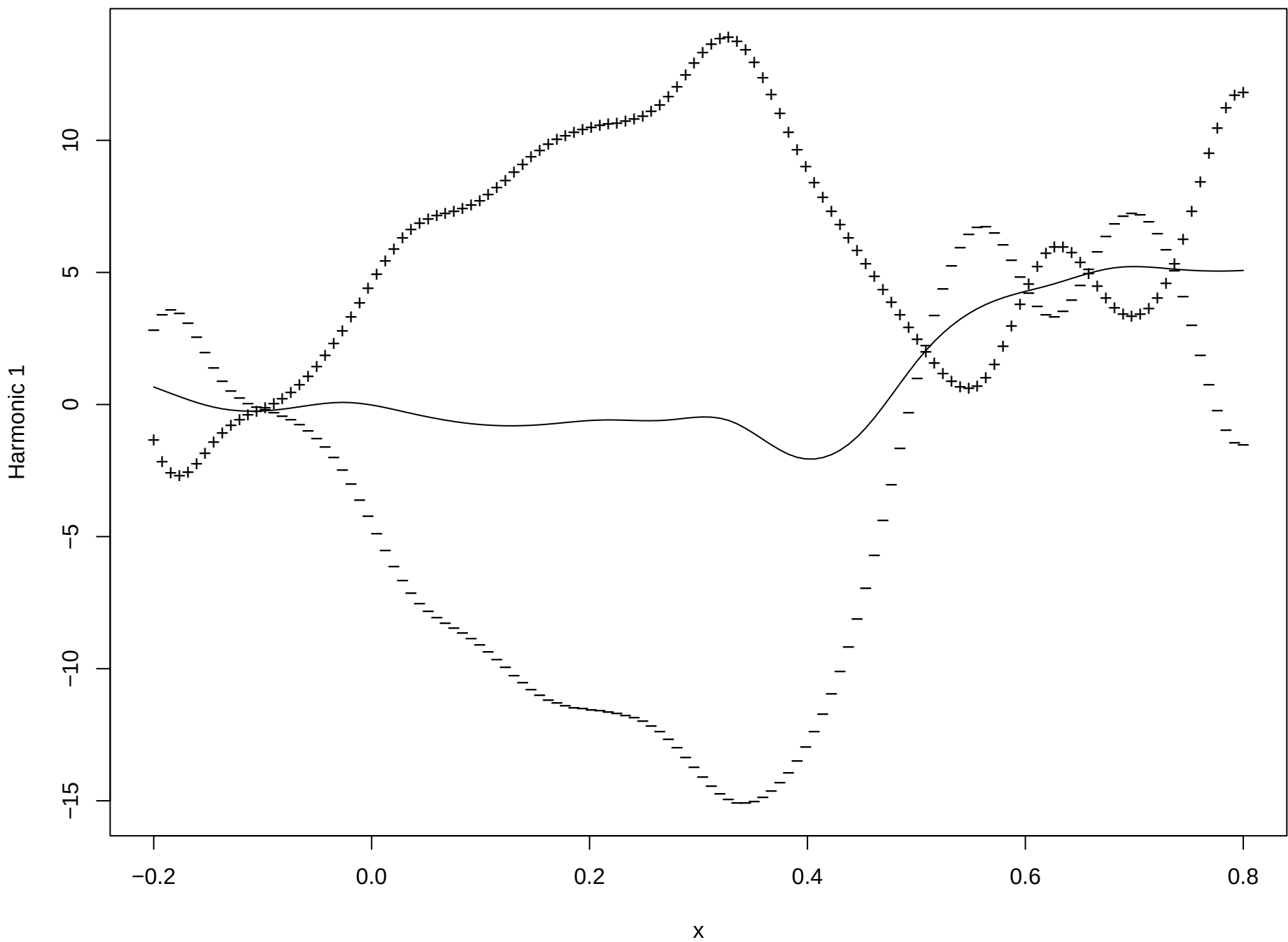
PCA function 1 (Percentage of variability 24.7 )
