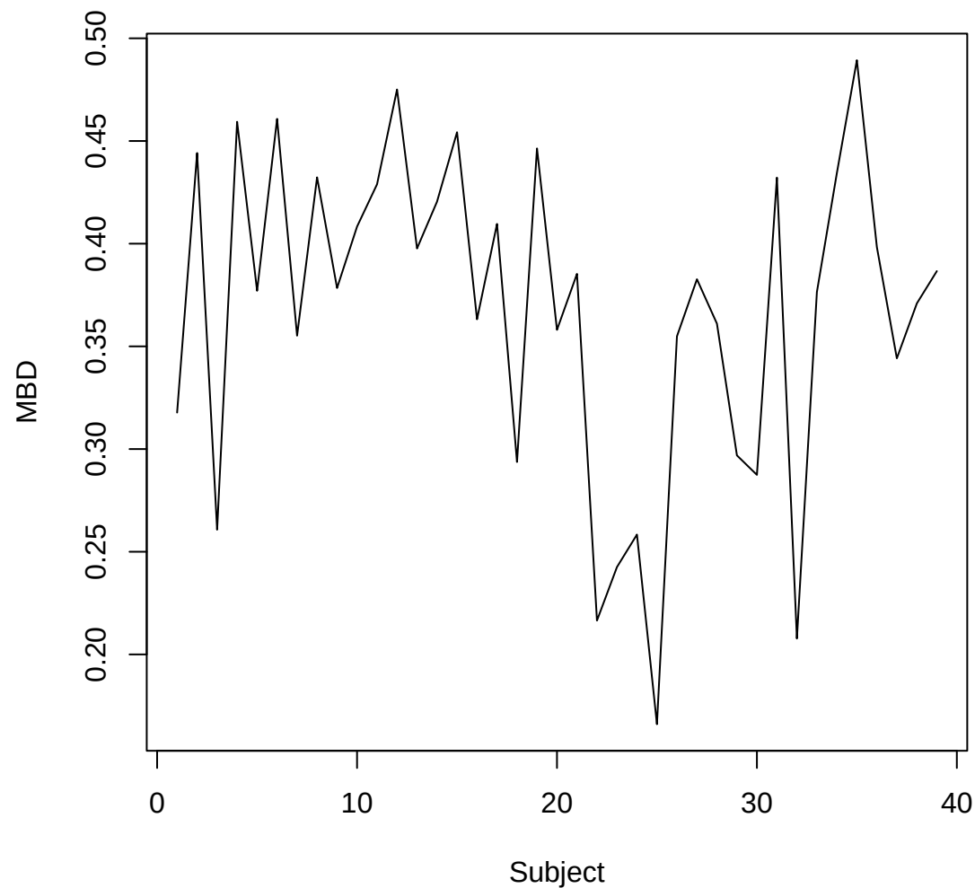
Modified Band Depth
