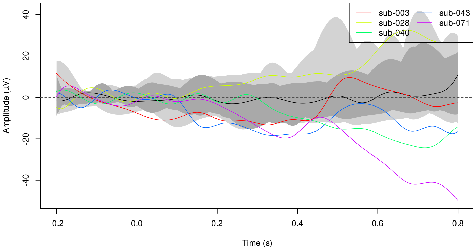
HDR Functional Boxplot, \alpha = (0.07, 0.50)
