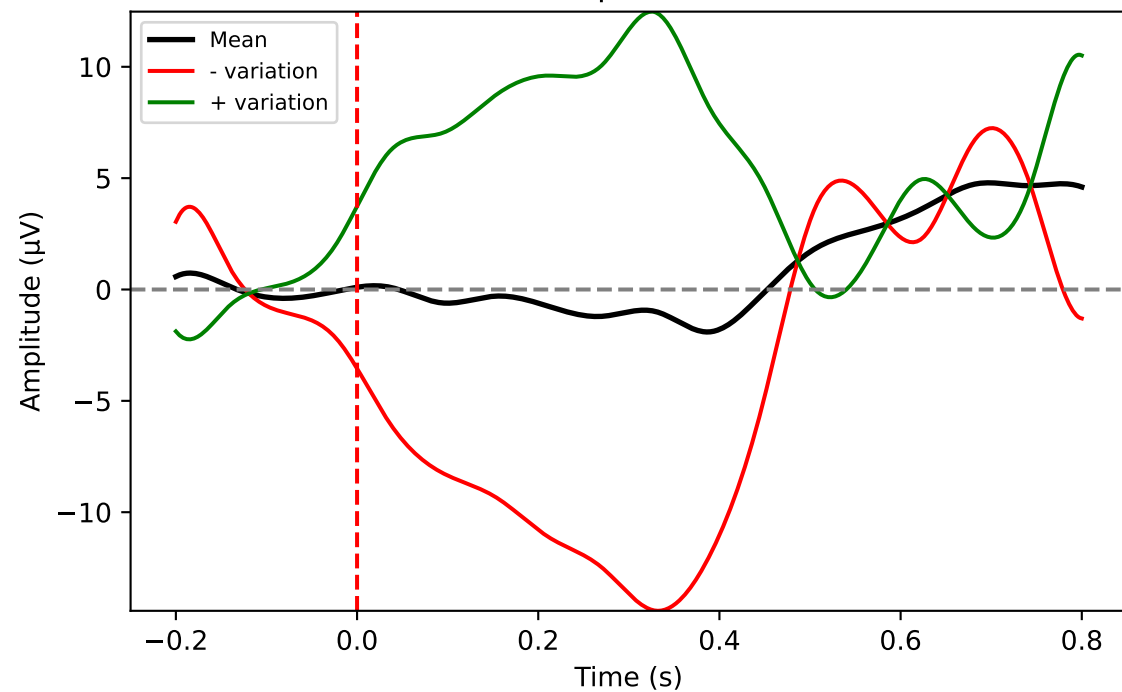
Rotated PC3 (Expl. variance: 18.7%)
