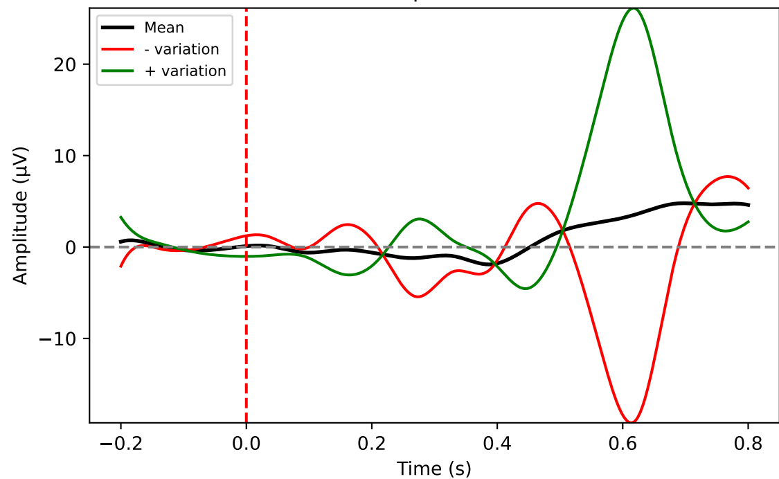
Rotated PC4 (Expl. variance: 19.3%)
