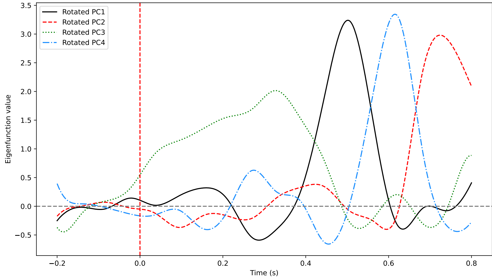
VARIMAX Rotated Harmonics
