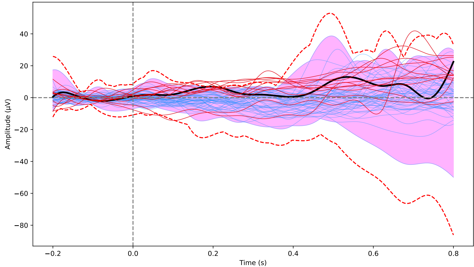
Functional Boxplot (BD2)
