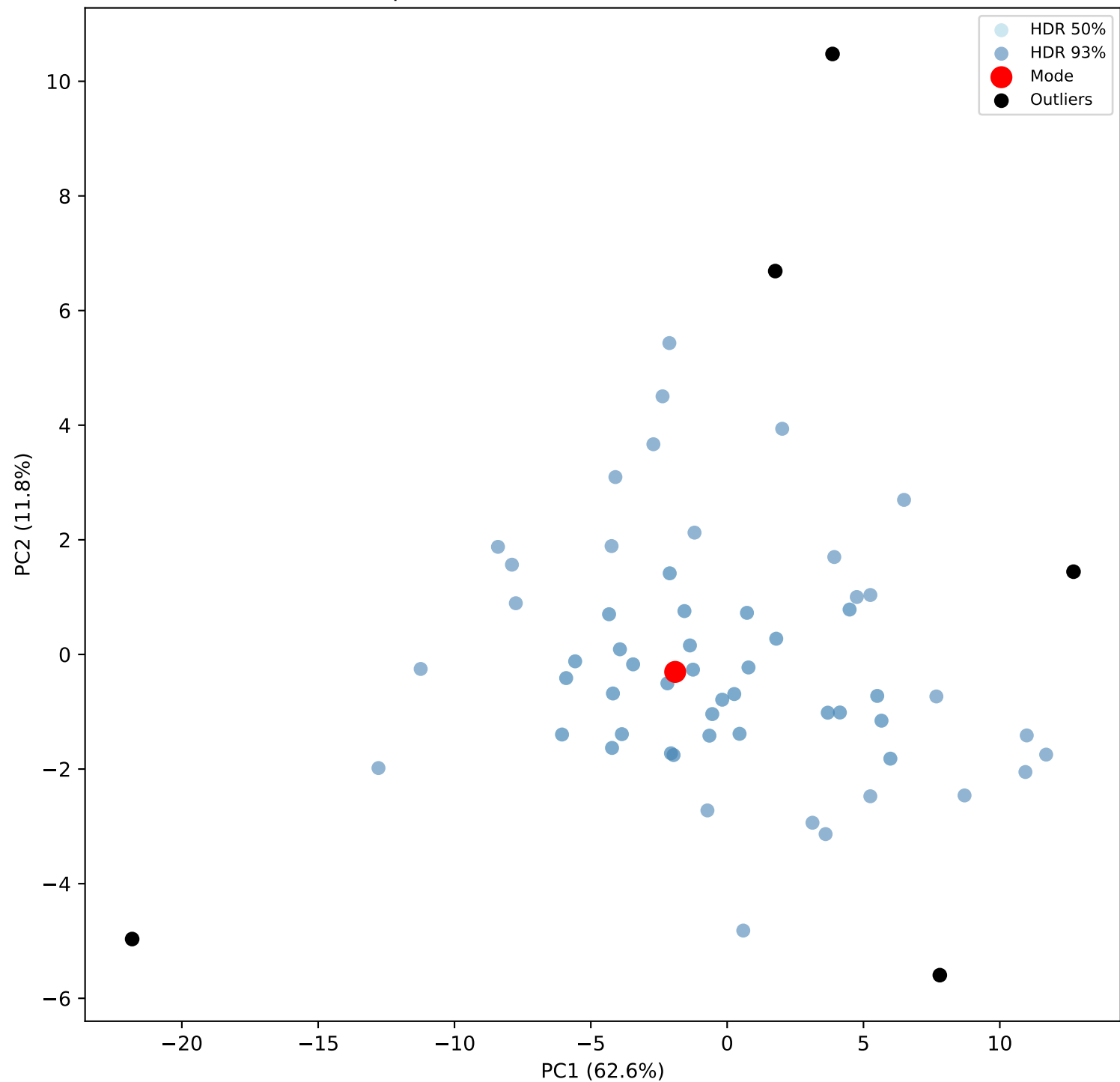
HDR Boxplot, \alpha=(0.07, 0.50) — Bivariate PCA Scores
