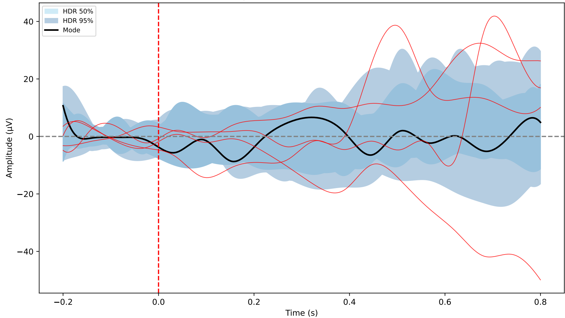
HDR Boxplot, \alpha=(0.05, 0.50) — Functional
