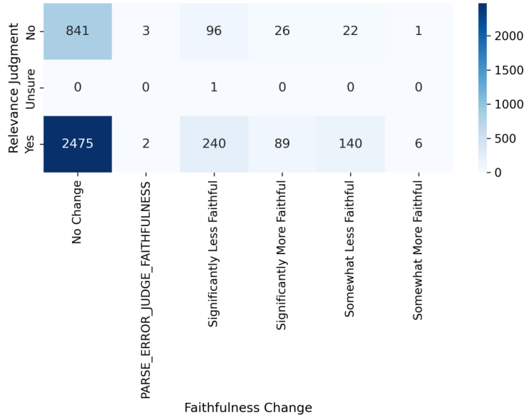
Relevance vs Faithfulness Cross-tabulation
