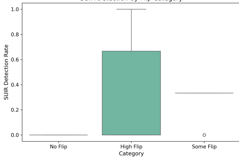
SUIR Detection by Flip Category
