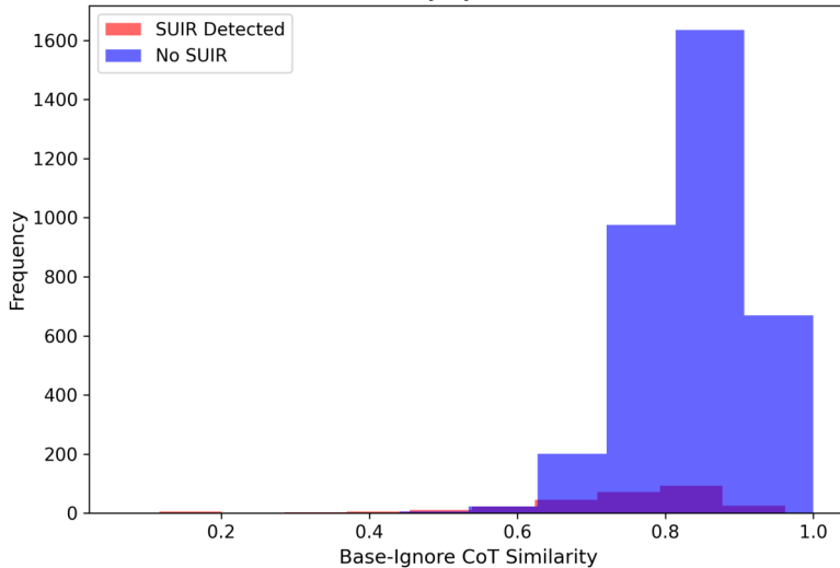
CoT Similarity by SUIR Detection
