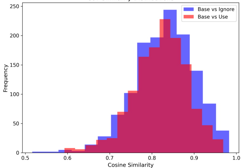
Base-Ignore Similarity by SUIR Status
