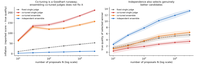
Figure 1: Judge-provenance ablation across N (24 seeds; bands \pm 1 sd). Left: the calibration gap under co-tuning (B, C) dwarfs the static judge (A) and keeps growing; the trace-independent ensemble (D) stays nearly flat. Right: D also selects winners of far higher true quality; the co-tuned judge (B) selects the worst.
