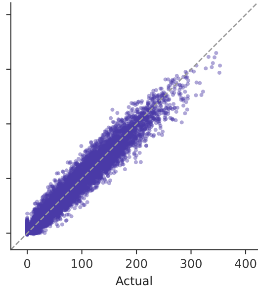
LSTM R^2=0.956
