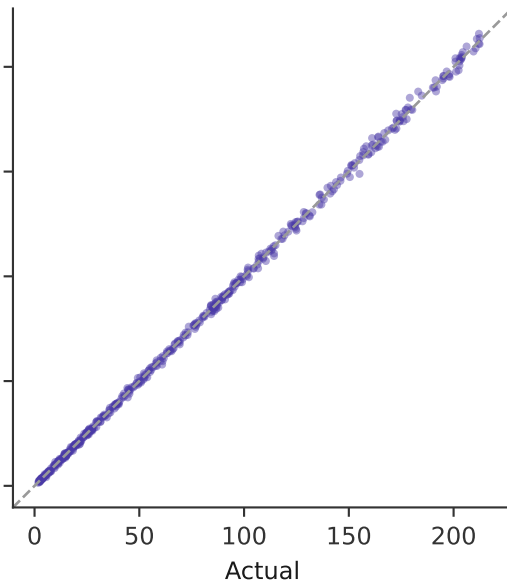
LSTM R^2=1.000
