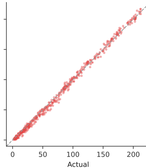
Chronos-Bolt (zero-shot) R^2=0.997
