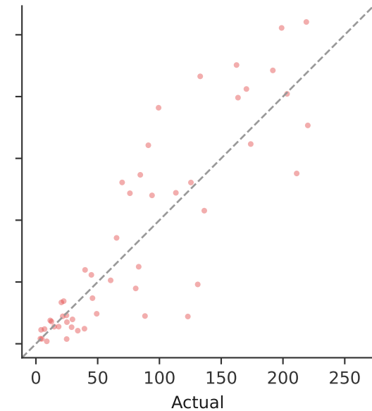
Chronos-Bolt (zero-shot) R^2=0.758
