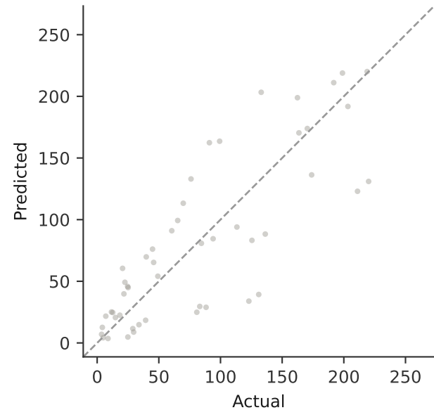
Naive Persistence R^2=0.673
