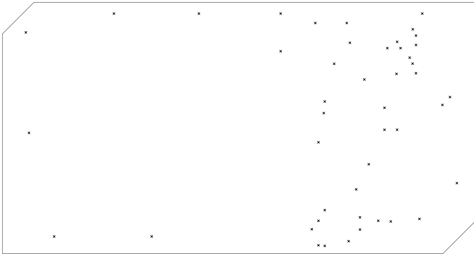
Drill Map: × 0.300mm / 0.0118" (46 holes)
